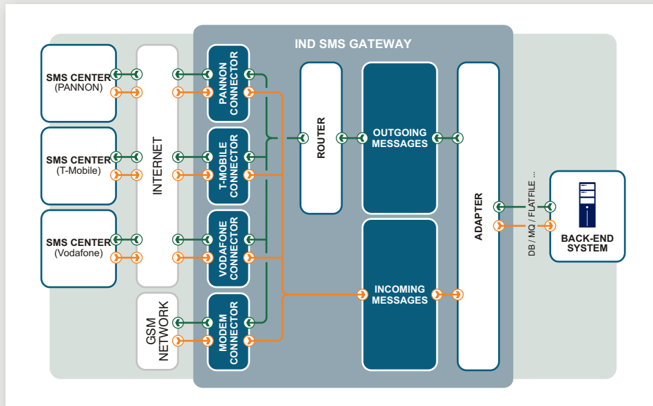
Figure 1: The SMS Gateway is also able to use standard industrial modem that acts as emergency channel in case of fatal communication problems.
